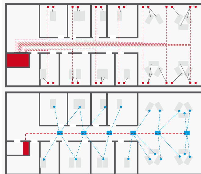
Typical plan of a typical office building
